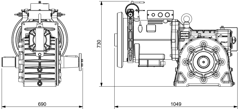
Figure 6 – Overall dimensions in the case of SH190 winch with SSB option without the drive pulley
