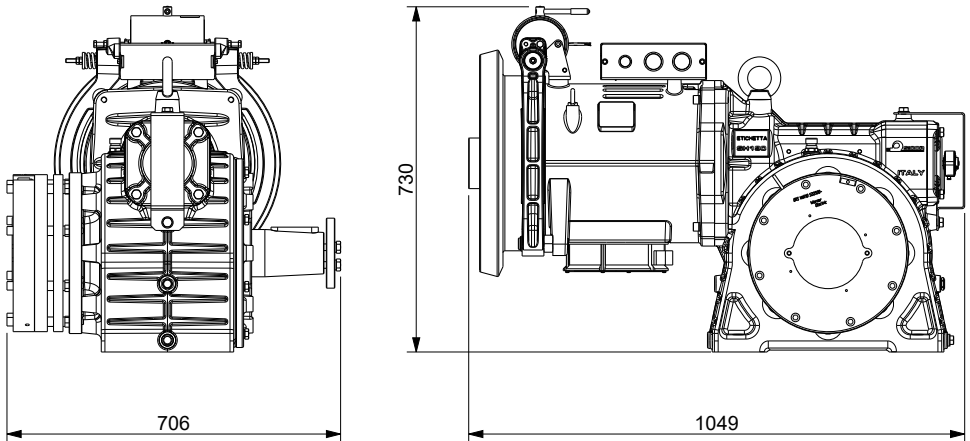
Figure 7 – Overall dimensions in the case of SH190 winch with emergency SSB (complete kit) without the drive pulley
