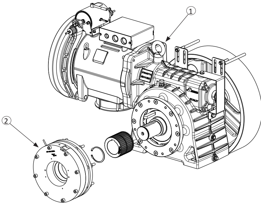
Figure 1 – SSB-SH190 winch assembly
