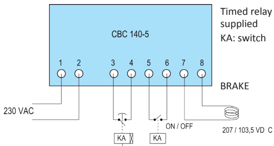
Figure 9 – Wiring diagram for the SSB power supply: KA switch (9A, 400V) and the relay are not included in the supply
