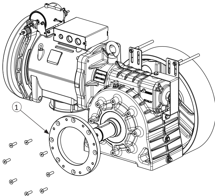
① SSB brake support flange code PIS0083
