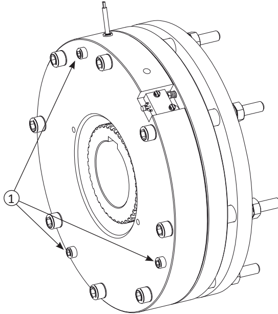
① SSB release screws
