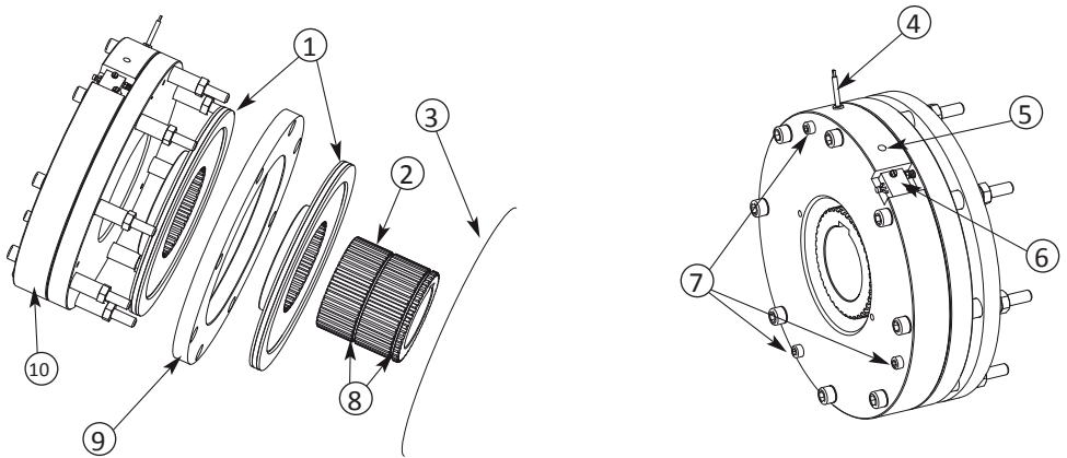
Figura 2 – Warner brake, type ERS VAR10-SZ2500/3000 (COD.: GEN0227), exploded drawing of the components and complete unit
