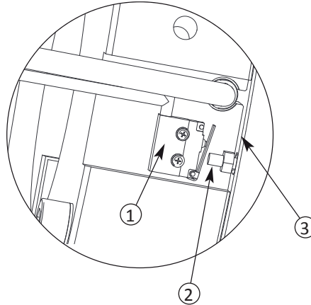
Figure 11 – Microswitch and adjustment screw
